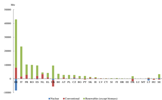
Graph I.1.4: Net change in installed generation capacity 2009-2013
