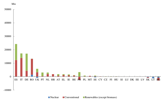
Graph I.1.3: Net change in installed generation capacity 2004-2008
