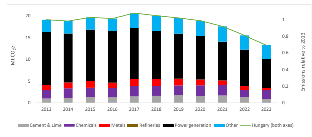
Graph A9.1: ETS emissions by sector since 2013
