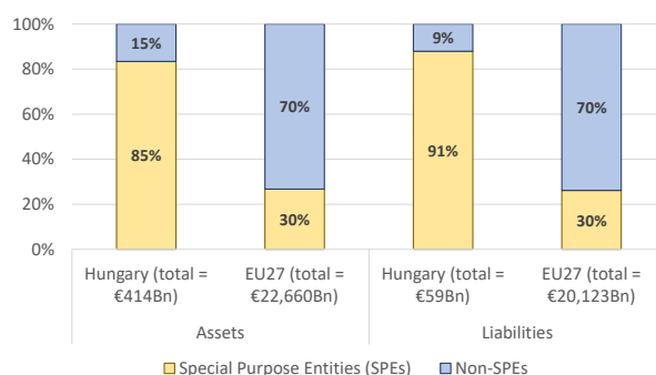
Graph A19.2: Stocks of assets and liabilities held through special purpose entities (SPEs) as a % of the respective total asset and liability stocks of foreign direct investment (FDI) in 2022
