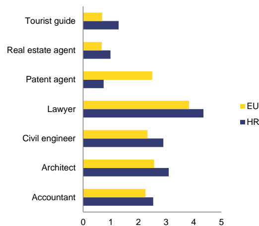
Graph 4.4.7: Restrictiveness indicator
