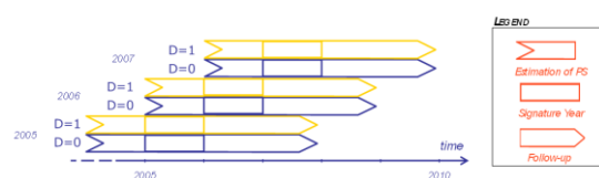
Graph 5.2: Sequential cohort design
