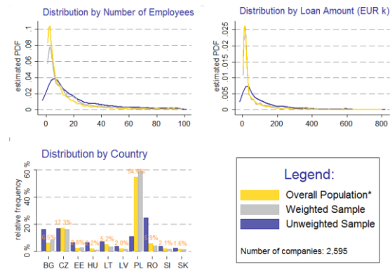
Graph 4.4: Distributions of treatment sample after reweighting
