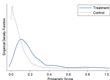
Graph 5.3: A graphical illustration of the PS model's predictive ability
