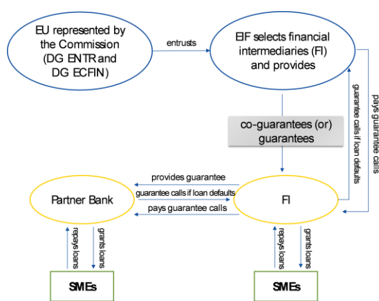
Graph 3.1: SMEG process under MAP
