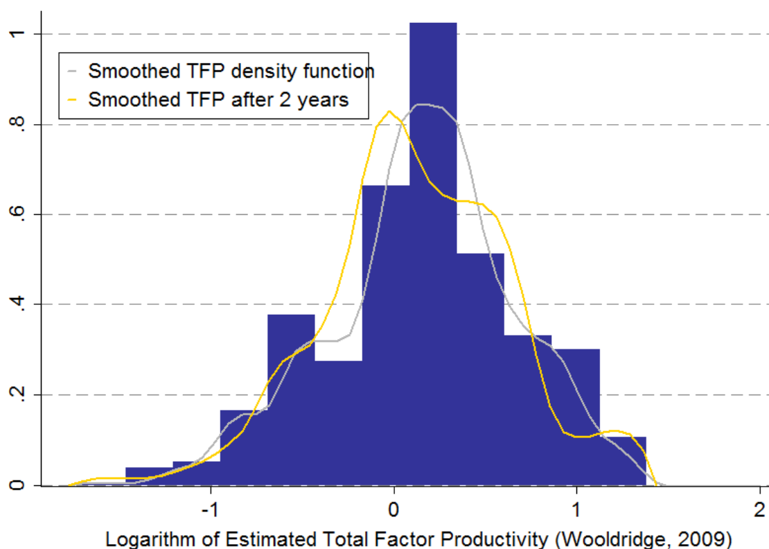
Graph A5.1: TFP distribution of MAP CESEE beneficiaries at signature date
