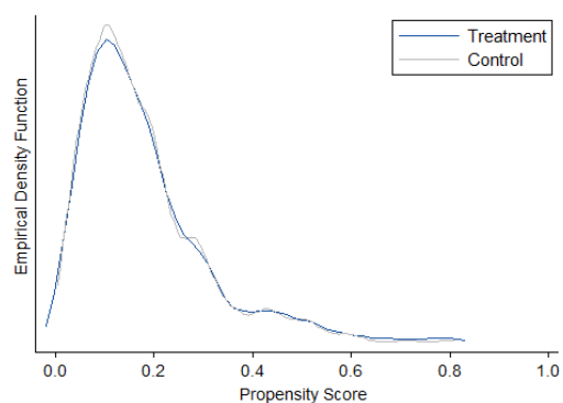
Graph 5.4: Empirical density functions of the propensity score after the NN-Matching
