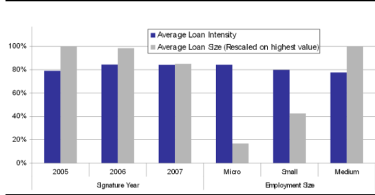
Graph 5.1: Observed heterogeneity of treatment
